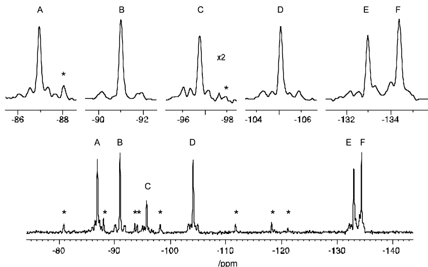
Figure 2. ^{183}\text{W}\{^{31}\text{P}\} NMR spectrum (12.5 MHz) of \text{TBA}_4[\text{PW}_{11}\text{O}_{39}\{\text{Ru}^{\text{V}}\text{N}\}] ( TBA-1 ) ( 1.2 \times 10^{-1} \text{ mol L}^{-1} in \text{DMF}/d_6\text{-acetone} ( T = 262 \text{ K} )). Bottom: full spectrum; top: abscissa expansion of the individual resonances. The signal marked by * correspond to [\text{H}_n\text{PW}_{11}\text{O}_{39}]^{(7-n)-} (ca 15%) and to [\text{PW}_{12}\text{O}_{40}]^{3-} (ca. 2%) impurities.
